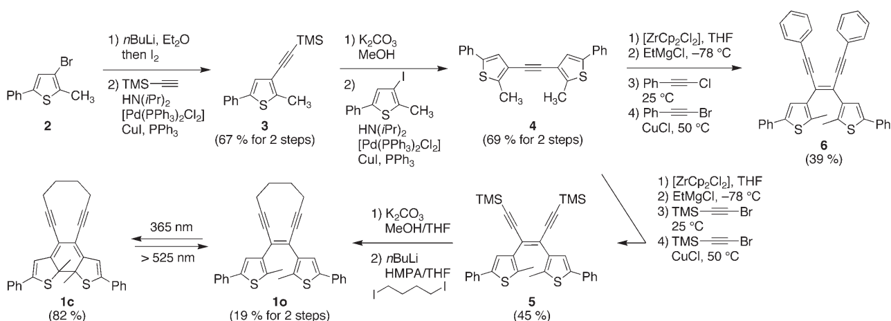
Scheme 2. Synthesis of DTE derivatives 1o and 6 with enediyne substructures. Cp = cyclopentadienyl, HMPA = hexamethylphosphoric triamide, TMS = trimethylsilyl.
