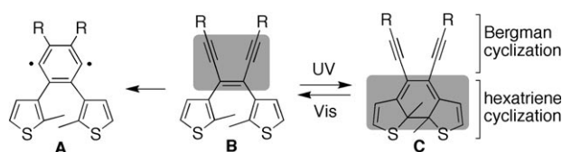
Scheme 1. Photochemical rearrangement used to create the enediyne structure. Only isomer B has the conjugated \pi system that undergoes the Bergman cyclization and produces the diradical A . Isomer C is inactive.
