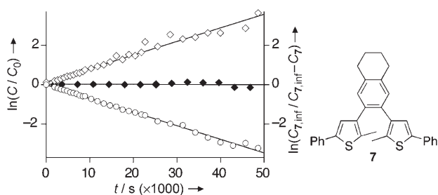
Figure 2. Changes in the concentrations of compounds 1o ( \circ ; initial concentration 4.22 \times 10^{-3} M), 1c ( \blacklozenge ; initial concentration 2.42 \times 10^{-3} M), and 7 ( \diamond ) as monitored by ^1\text{H} NMR spectroscopy. The concentrations are measured by comparing the integrated areas under the peaks for each compound against p -nitroanisole as an internal standard and are normalized for easier comparison. The left vertical axis corresponds to the disappearance of compounds 1o and 1c , where C is the concentration of 1o or 1c at a given period of time and C_0 is initial concentration of each compound. The right vertical axis corresponds to the appearance of compound 7 , where C_7 is concentration at a monitored period of time and C_{7,\text{inf}} is the final concentration of 7 .
