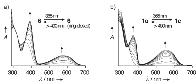
Figure 1. Changes in the UV/Vis absorption spectra of compound 6 (a) and 1o (b) upon irradiation with \lambda = 365 nm (benzene solutions, 2.65 \times 10^{-5} M and 8.22 \times 10^{-5} M for 6 and 1o , respectively). Spectra were recorded every 10 seconds until a 90-second period (for 6 ) and a 120-second period (for 1o ) were completed.
